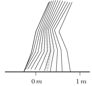
Fig. 6. Stick animation of robot taking one step from left to right. Note that the stance leg is dotted.
