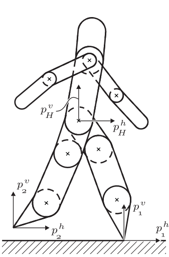
Fig. 1. A higher DOF robot model. Cartesian coordinates are indicated at the hips and the leg ends.
