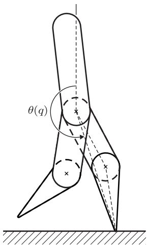
Fig. 3. Example \theta(q) measured between the vertical and the line connecting the hips and the stance leg end.
