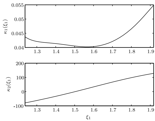
Fig. 9. Constituent functions of the zero dynamics for the example.
