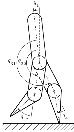
Fig. 2. Schematic of the 5-link robot considered with measurement conventions.
